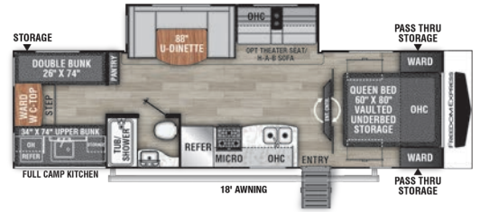
292 BHDS / Exterior Length 33' 4"
