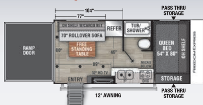
17 BLSE / Exterior Length 20' 3"
