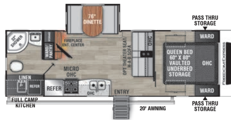
252 RBS / Exterior Length 29' 7"
