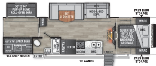
310 BHDSLE / Exterior Length 35' 6"
