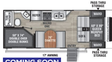
22 SE / Exterior Length 24' 11"
