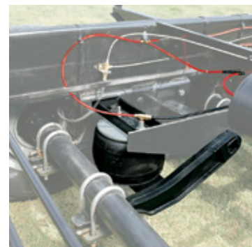
O Smooth out the road with this independent Air Ride suspension system, acting in tandem with a torsion axle, that puts each tire on its own active cushion of air — filling and releasing as needed.
