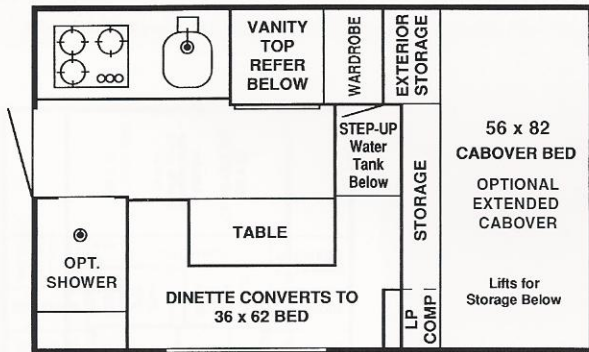
TC800 with Optional Shower.
