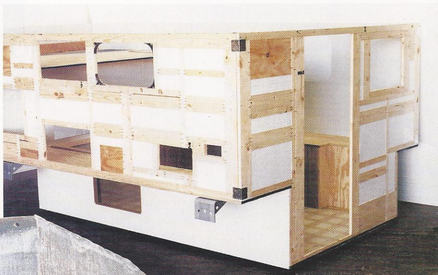
Pop-up standard insulation and body
