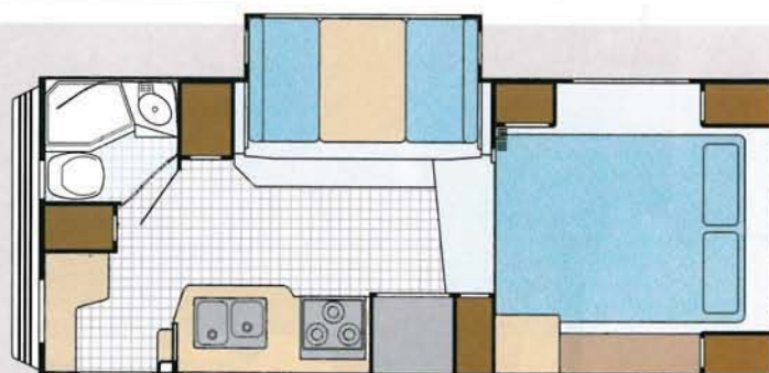
Lance 1161 — 11' 11"
