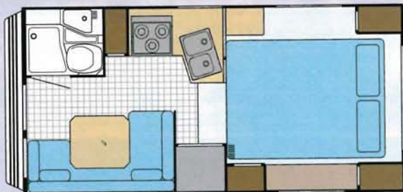
Lance 820 – 8' 11"
