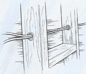
24 Metal sleeves in wall studs protect all 110 volt wiring.
