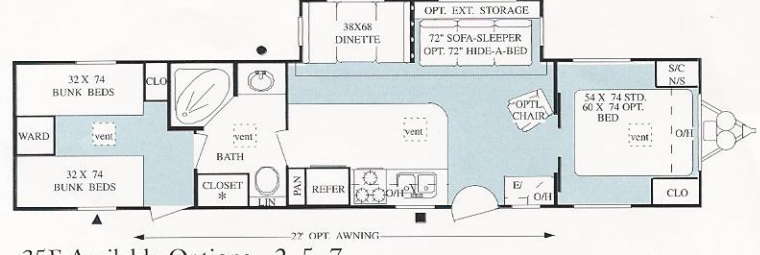
35F Available Options - 2, 5, 7
