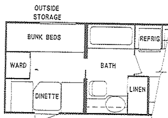
Option Walk-Thru Bath/Rear Dinette (Model 3511)
