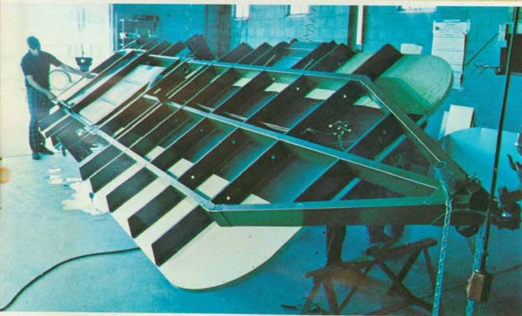
Avion has a tremendously strong triple-beam frame of heavy duty steel, including a rugged center beam for added support. Frame members are 5" deep (6" on 31 ft.).
